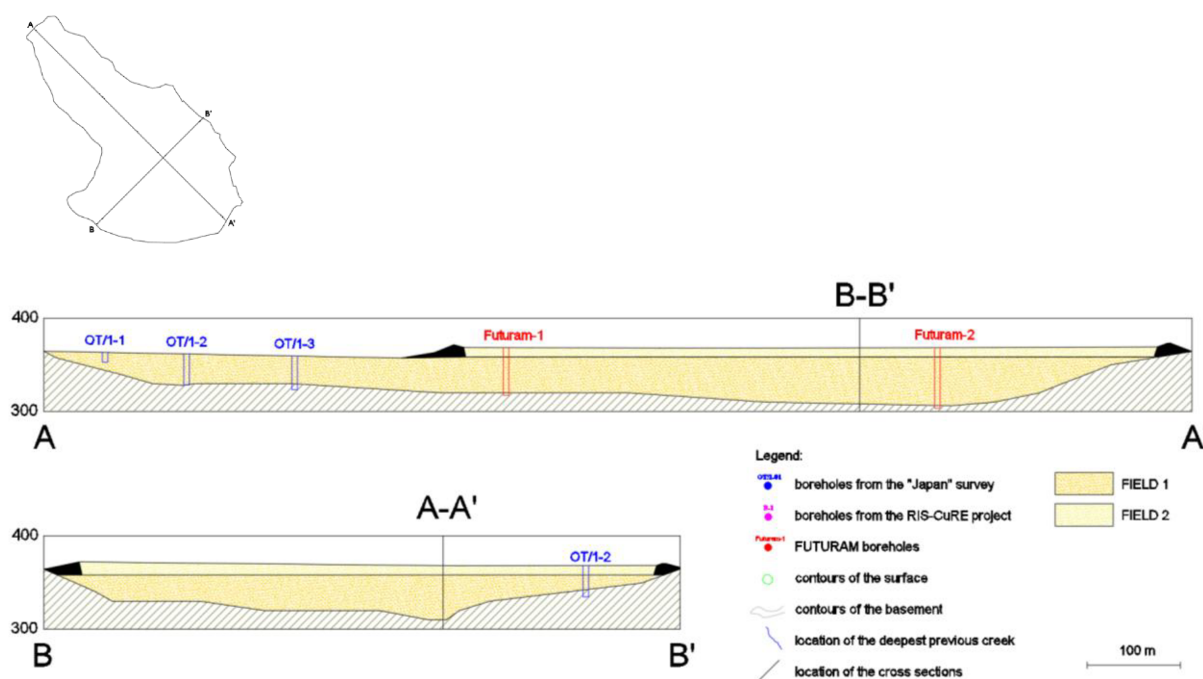
Figure 18: Geological model of the tailings dam, shown on two perpendicular cross sections. Higher grade material in Field 1, which outcrops on the NW part, is covered by the lower grade materials of Field 2. Descriptive statistical parameters of the chemical analyses are presented for both field separately in Table 9.
