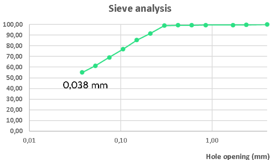
Figure 21: Sieve analysis of composite sample from Field 1 [18].
